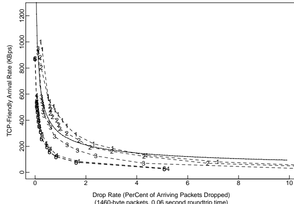
Figure 9: TCP-friendly bandwidth for a 60-ms roundtrip time and 1460-byte packets.
