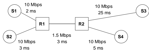
Figure 13: Simulation network.
