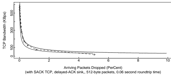
Figure 10: TCP bandwidth vs. steady-state drop rate, for SACK TCP with a delayed-ACK sink, a 60-ms roundtrip time and 512-byte packets.
