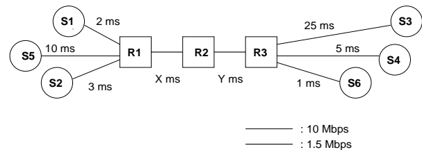
Figure 6: Simulation network.
